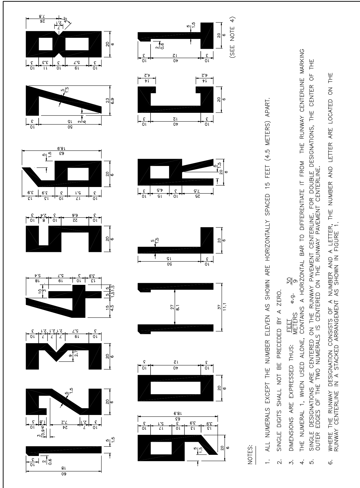
Figure 4. Runway Designation Numerals and Letters
