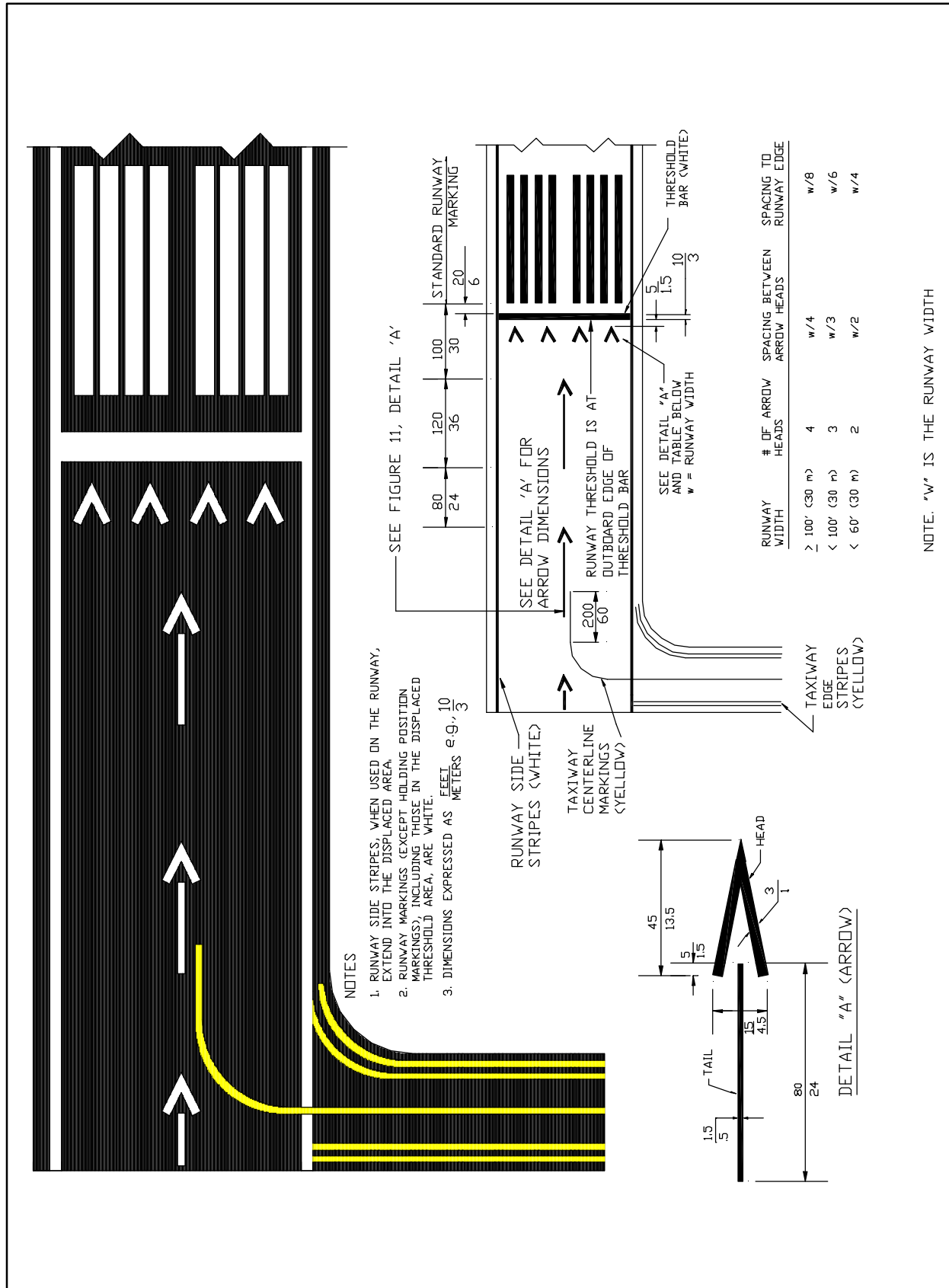
Figure 5. Displaced Threshold Markings
