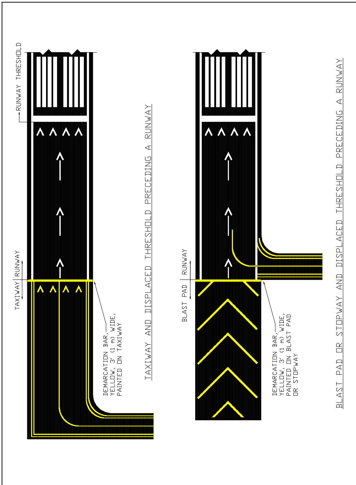
Figure 8. Marking for Blast Pad or Taxiway Preceding a Displaced Threshold
