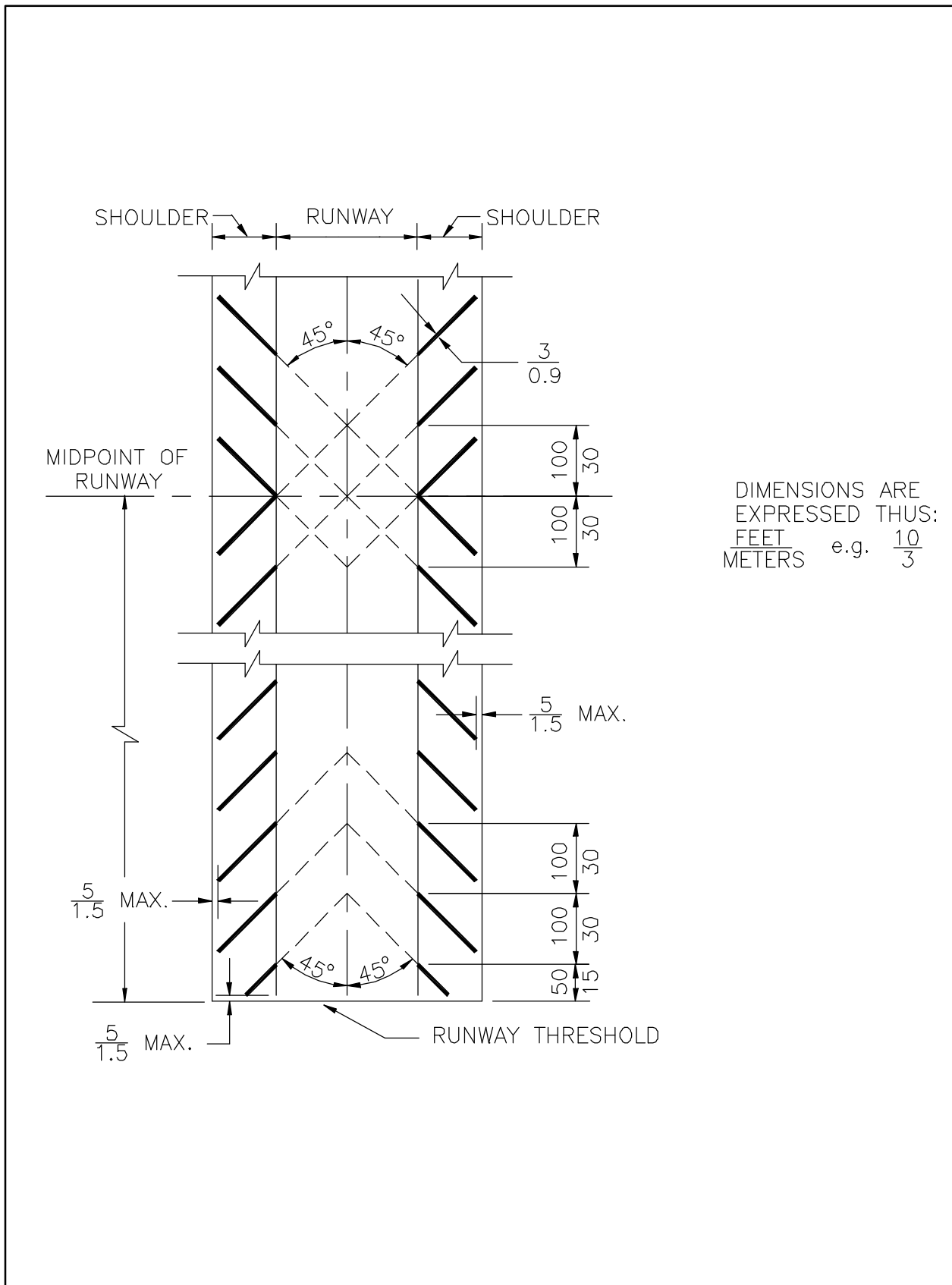
Figure 9. Runway Shoulder Markings
