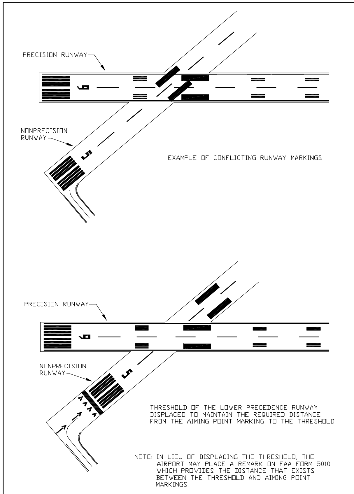
Figure 3. Example of Conflicting Markings on Crossing Runways
